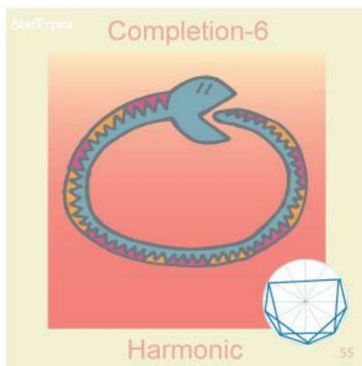
StarType #55, 6-Noviles
