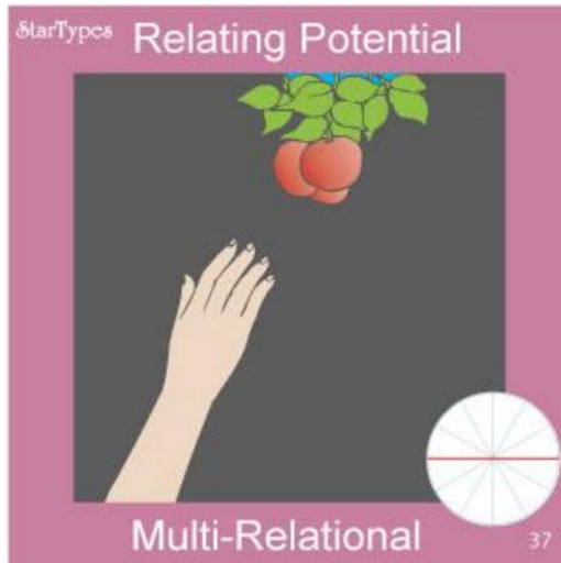
StarType #37, Oppositions
