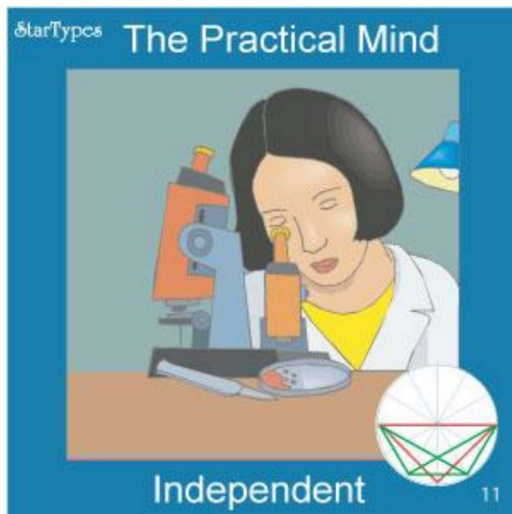
StarTypes #11, T-Basket
