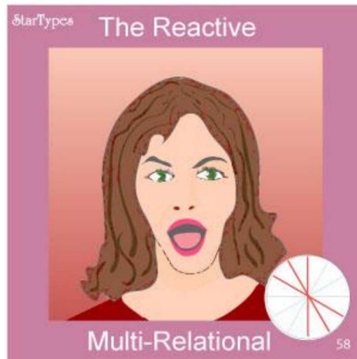
StarType #58, Splay
