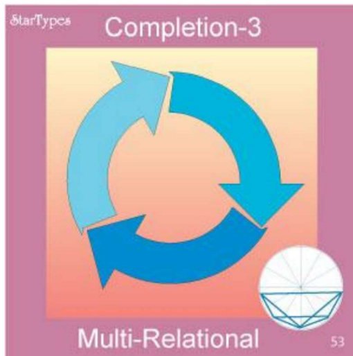
StarType #53, 4-Noviles
