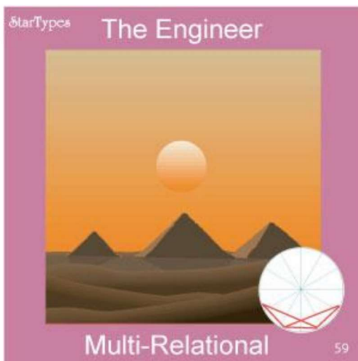
StarType #59, 3-45s
