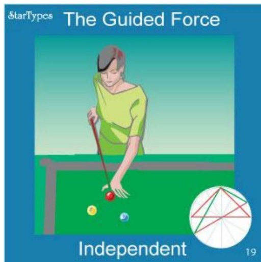
StarType #19, Nutcracker
