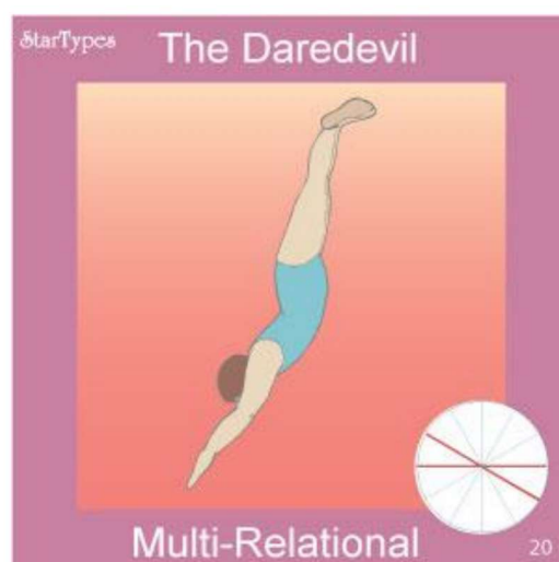
StarType #20, Warrior
