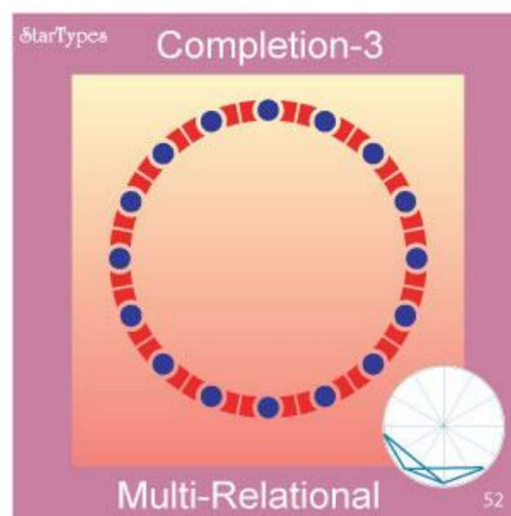
StarType #52, 3-Noviles
