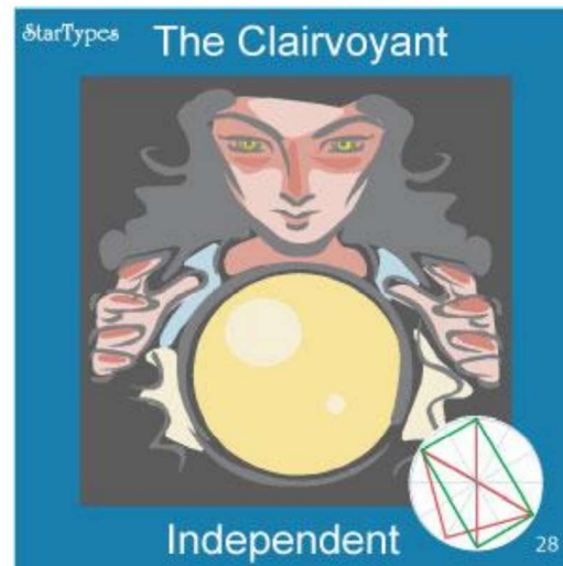
StarType #28, T-Rectangle
