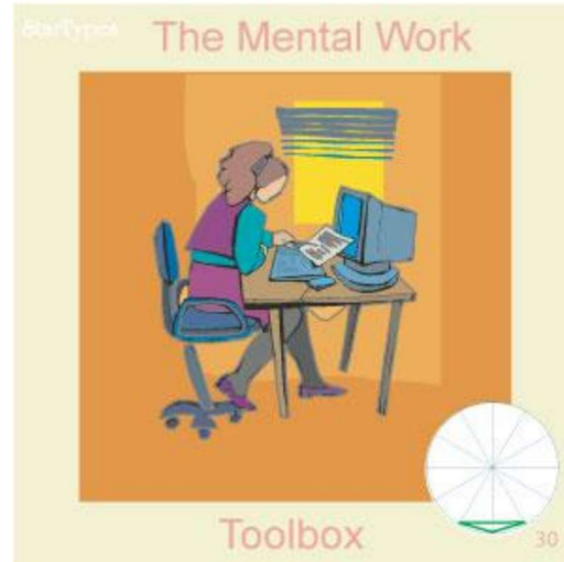
StarType #30, 2-30s 60
