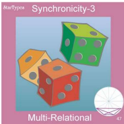
StarType #47, 3-Septiles
