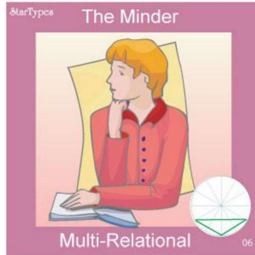
StarType #6 2-60s
