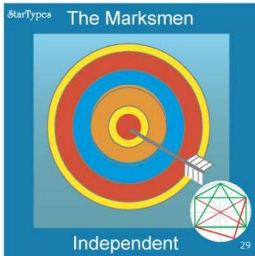
StarType #29, T-Seer
