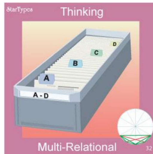
StarType #32, 4-30s 120
